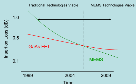
Study showing the transition from traditional technology to MST based RF switches
